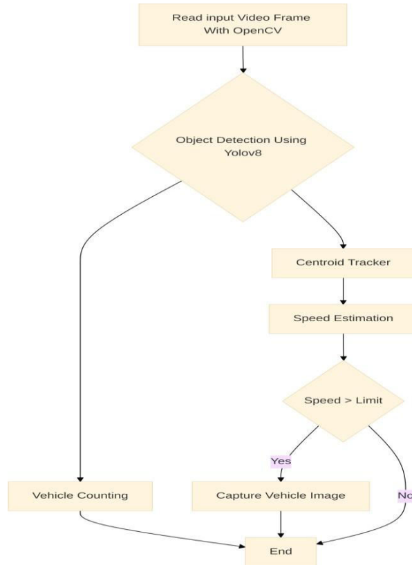
Fig 3.2: Flowchart of Vehicle Detection and Speed Estimation
