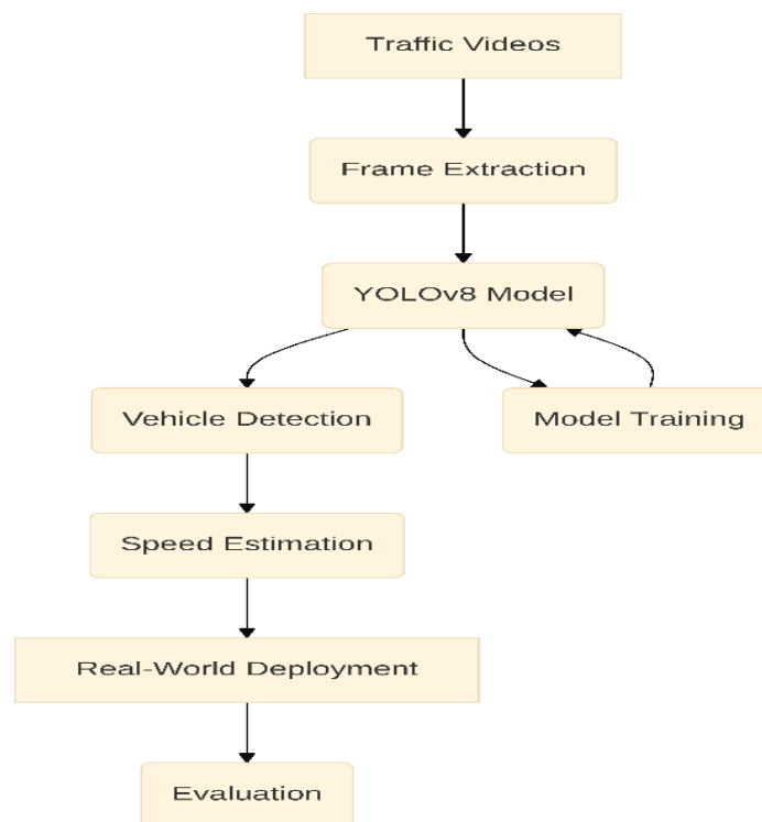
Fig 3.1: System Architecture
