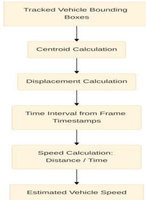
Fig 3.4: Speed Estimation Model
